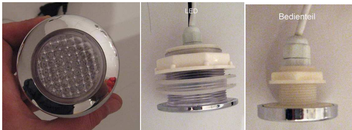
LED (Frontansicht)
